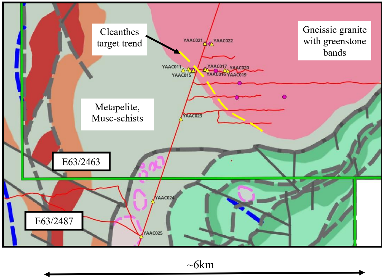
Fig. 6. Location of May AC holes on interpreted geology (Fig.1) – Cleanthes Magenta circles: historical RAB anomalies > 0.1 g/t Au and > 0.5 g/t Au (ASX: CUL; 28-1-2025)
