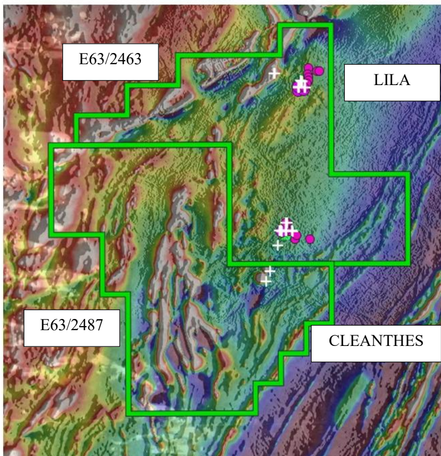
Fig. 2 TMI1VD Magnetics image White crosses = Cullen May AC holes: YAAC series Magenta circles: historical RAB anomalies: > 0.1 and > 0.5 g/t Au (ASX: CUL; 28-1-2025)
