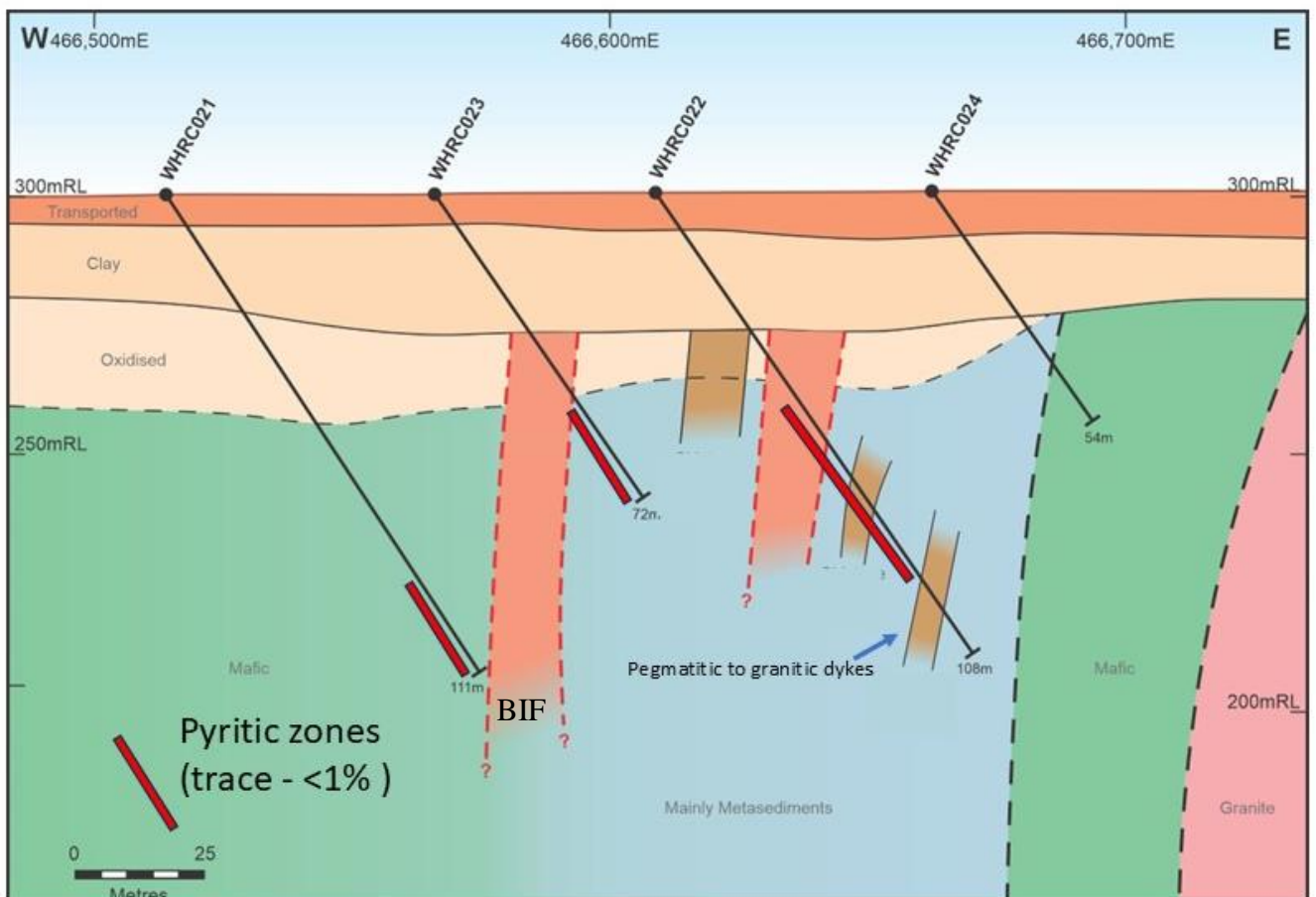
Fig. 12. x-section Rupert, WHRC021 – WHRC024
