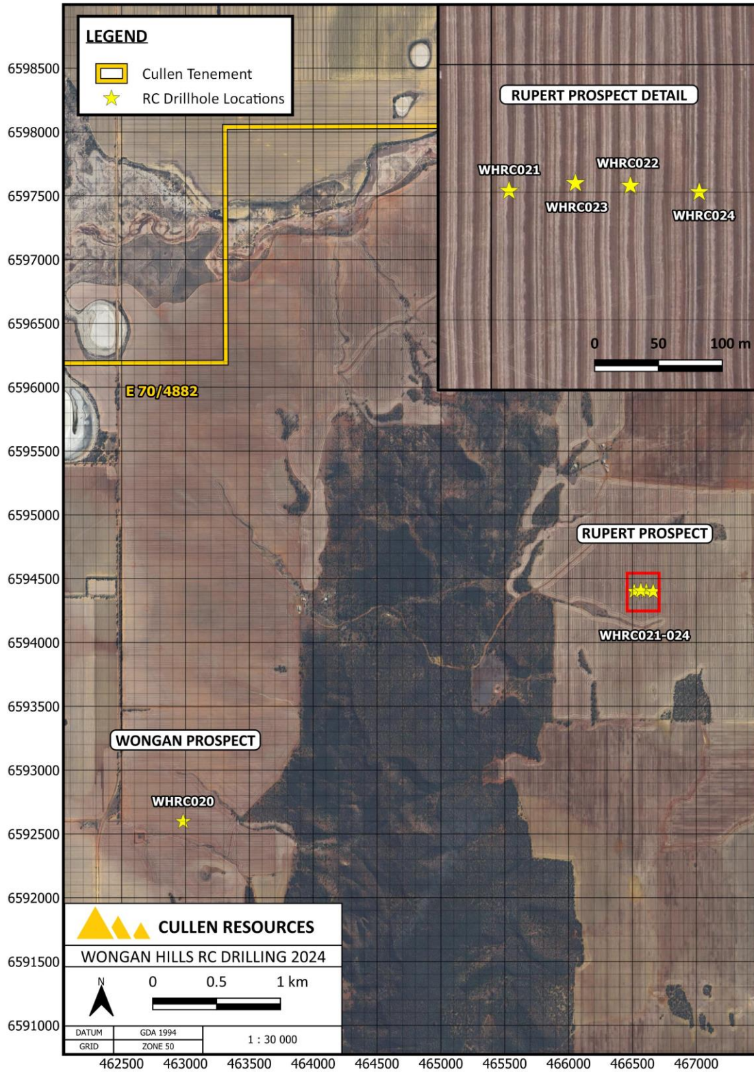
Fig. 8. Location plan for RC drilling, December 2024. Detail of locations at Rupert in Inset.
