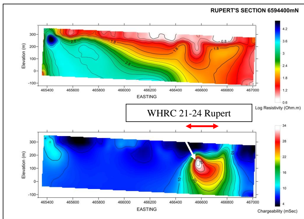
Fig. 2. Trial IP survey Chargeability and Resistivity sections, 6594400mN (and see Fig.10)
