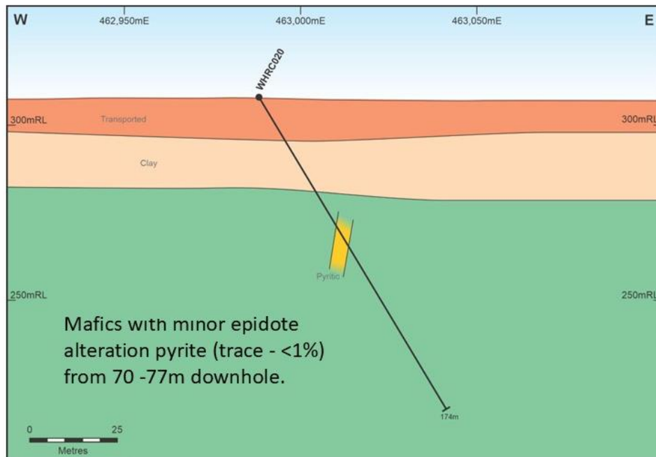
Fig. 11 x-section Wongan, WHRC020
