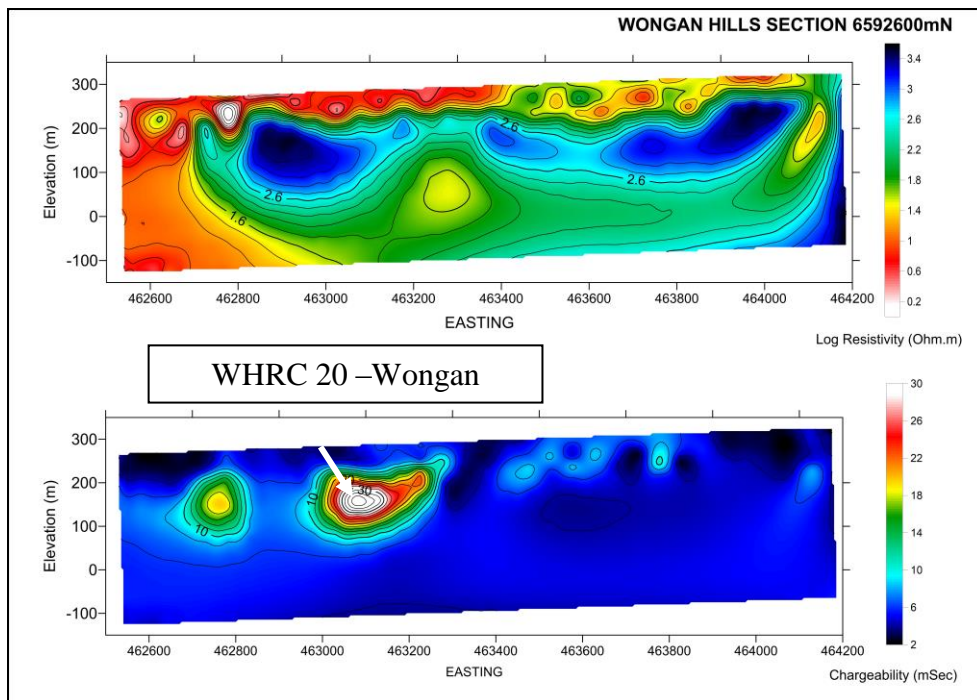
Fig. 1 Trial IP survey Chargeability and Resistivity sections, 6592600mN (and see Fig.9)
