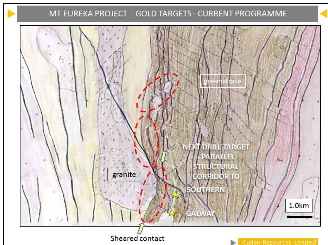
Fig.1. Location of new gold targets in the vicinity of the Southern-Galway gold zone.
