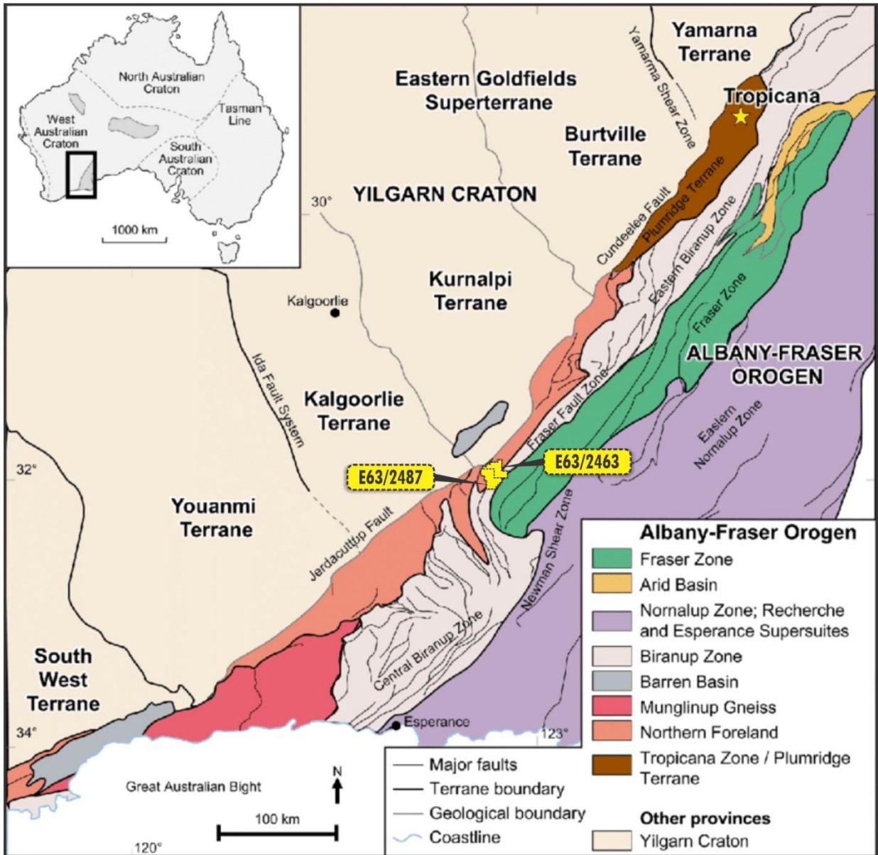
Fig.1. Regional geological map of the Albany-Fraser Orogen with respect to the eastern margin of the Yilgarn Craton, W.A. The position of the Yardilla project tenements is shown (figure modified after Spaggiari et al., 2011: The geology of the East Albany-Fraser Orogen: a field guide; GSWA Record 2011/23).
