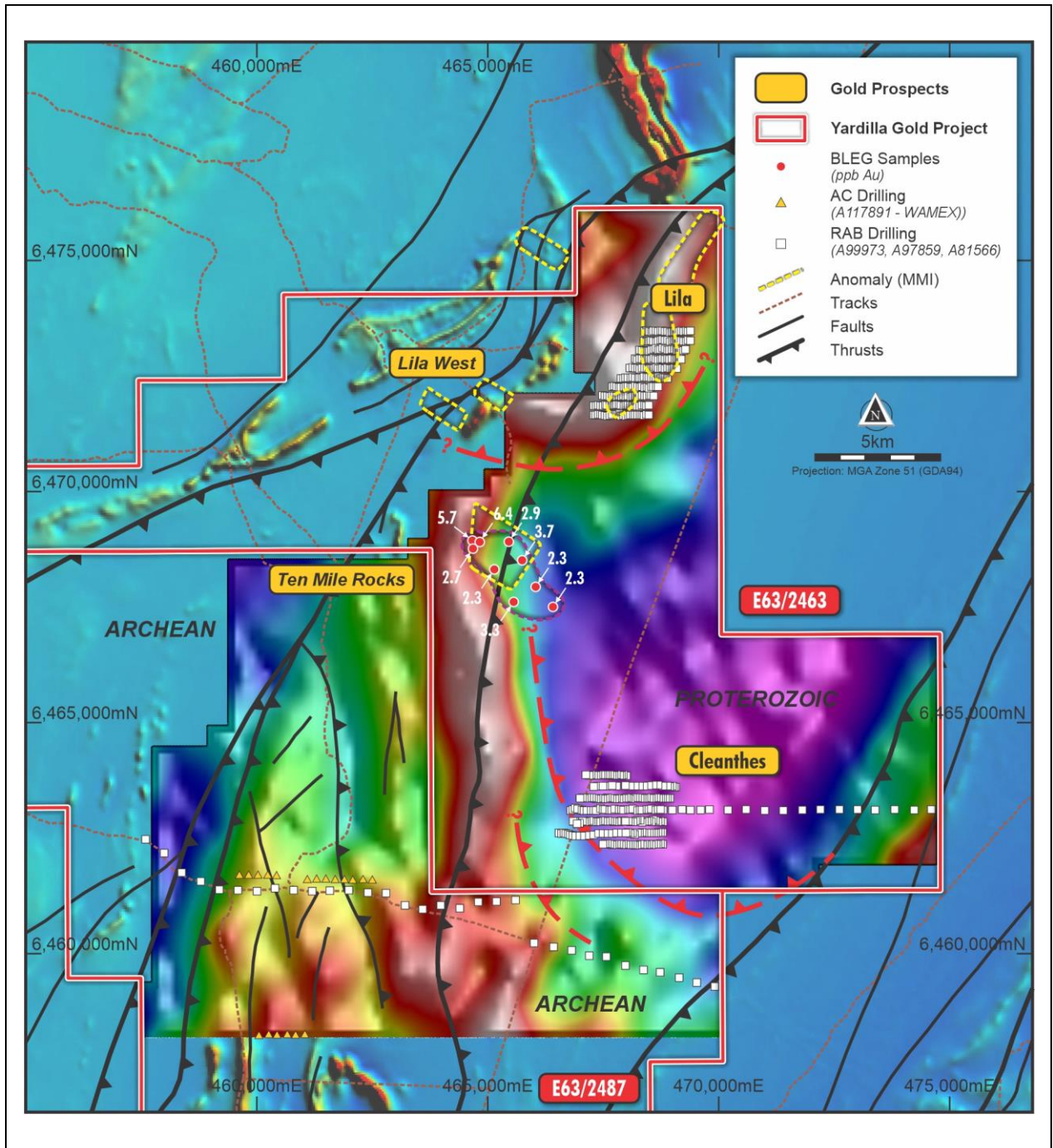
Fig. 2. Gravity image (from WAMEX A99973) superimposed on mag image (from Fig.4) underlines focus of soil anomalies along the thrust boundary between low density Proterozoic granitic gneiss, and the Archaean to the north, west and south.
