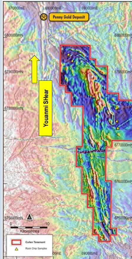
Magnetics Image
